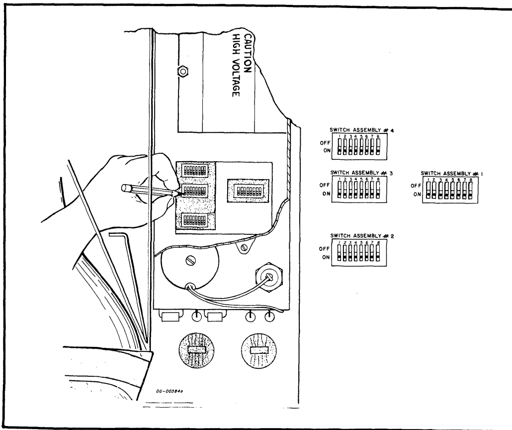
Figure 3-1 Setting the DGC Display Selection Switches
